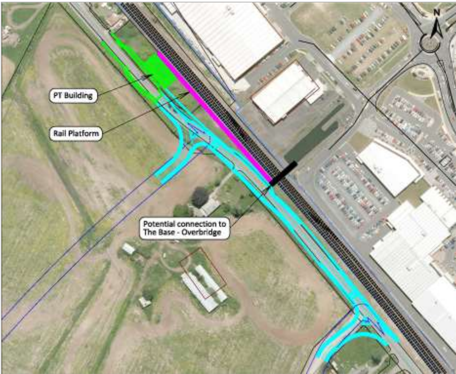
Figure 3.6.2b: The Base Site Layout Development Complex
