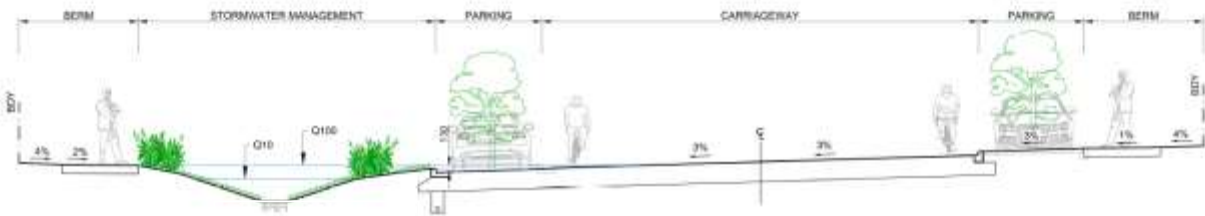
Figure 3.6A-5 INDICATIVE COLLECTOR ROAD CROSS SECTION WITH SIDE SWALE
