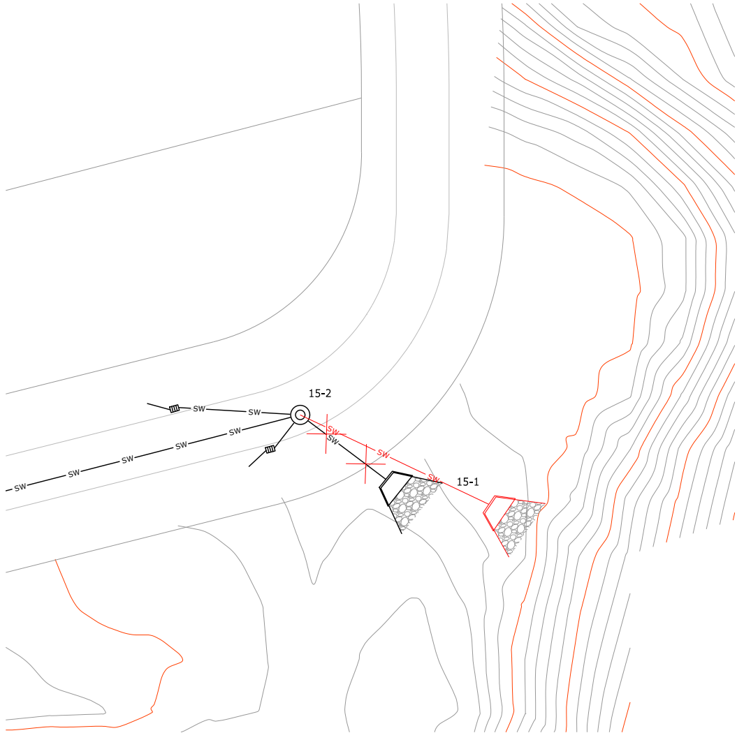
9 HEADWALL LAYOUT PLAN SK293 SCALE 1:250-A1 1:500-A3
