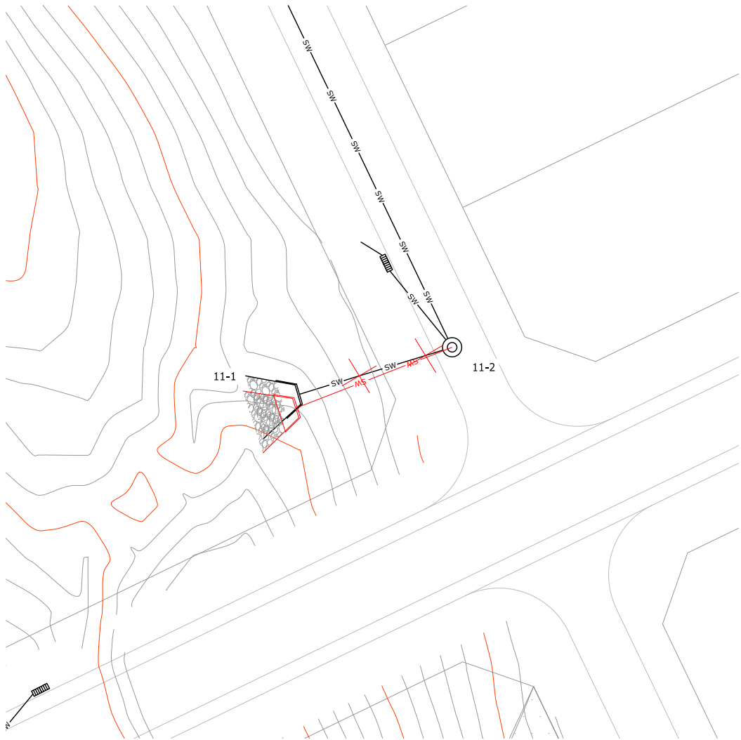
15 HEADWALL LAYOUT PLAN SCALE 1:250-A1 1:500-A3
