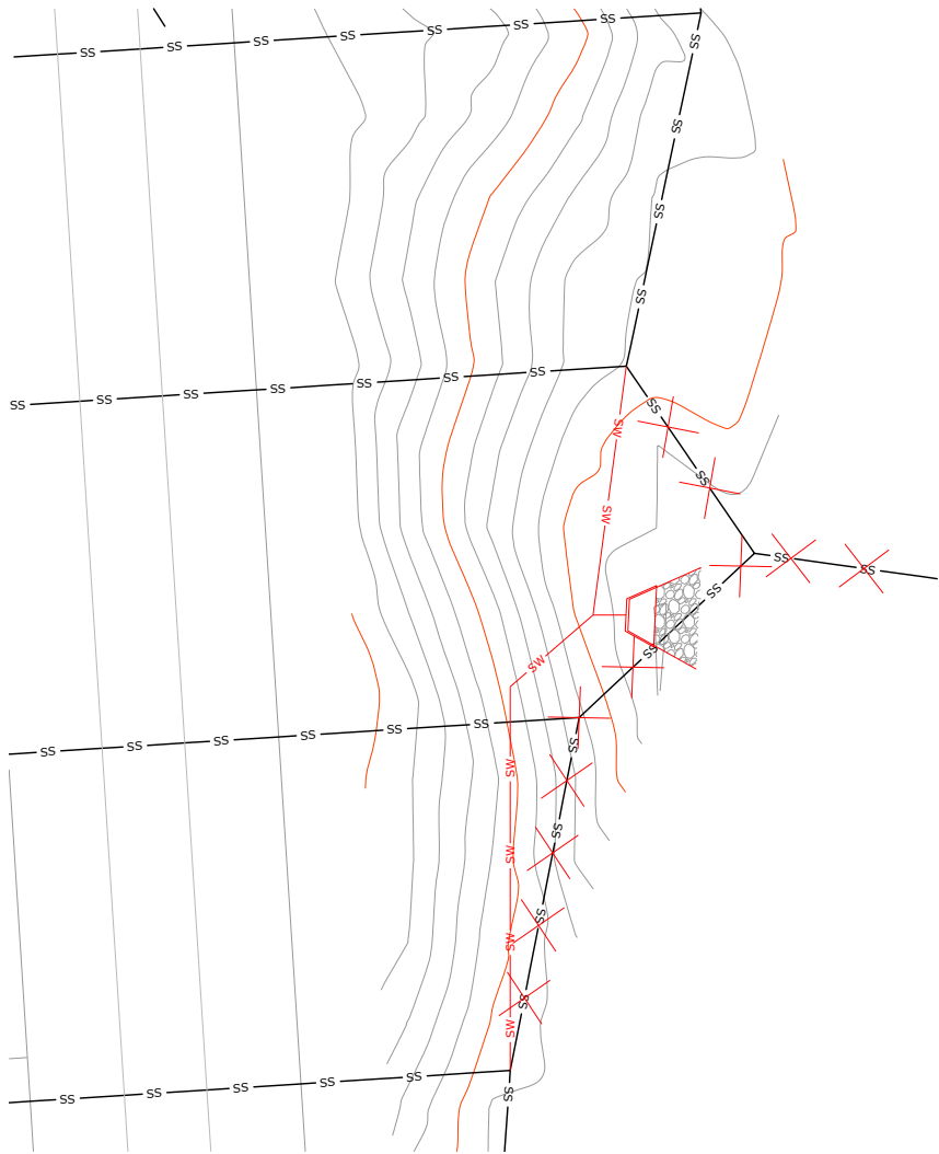
4 HEADWALL LAYOUT PLAN SK291 SCALE 1:250-A1 1:500-A3
