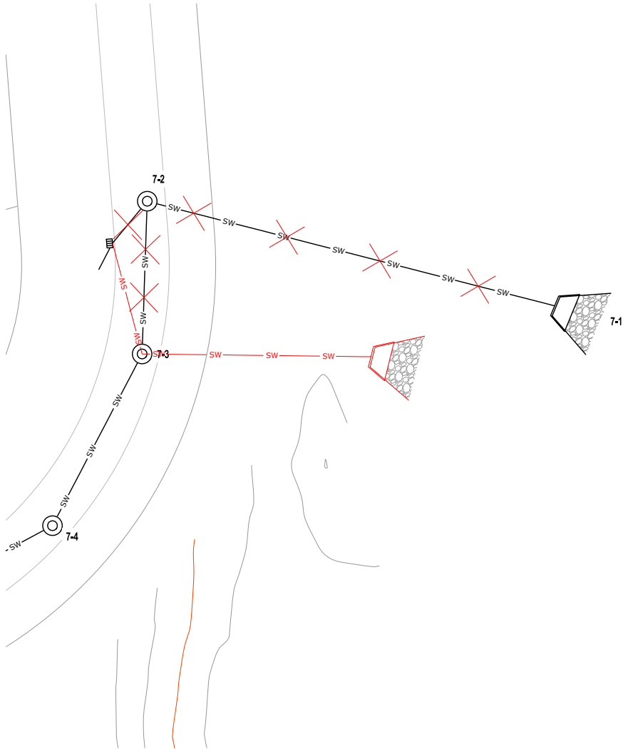
3 HEADWALL LAYOUT PLAN SK291 SCALE 1:250-A1 1:500-A3
