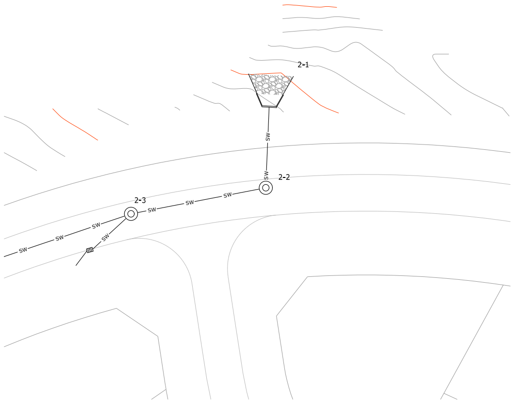
2 HEADWALL LAYOUT PLAN SK291 SCALE 1:250-A1 1:500-A3
