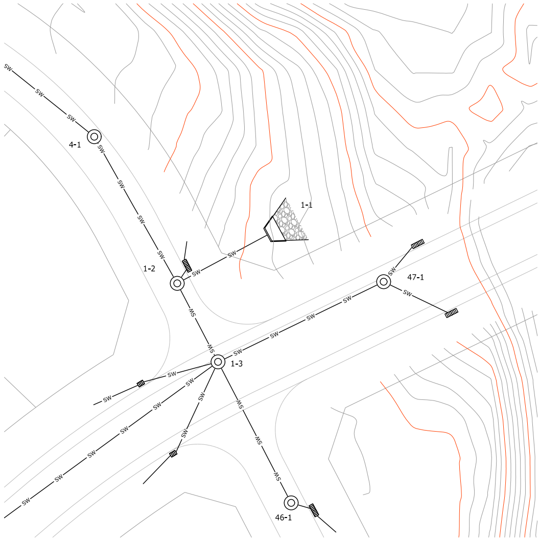
13 HEADWALL LAYOUT PLAN SK295 SCALE 1:250-A1 1:500-A3
