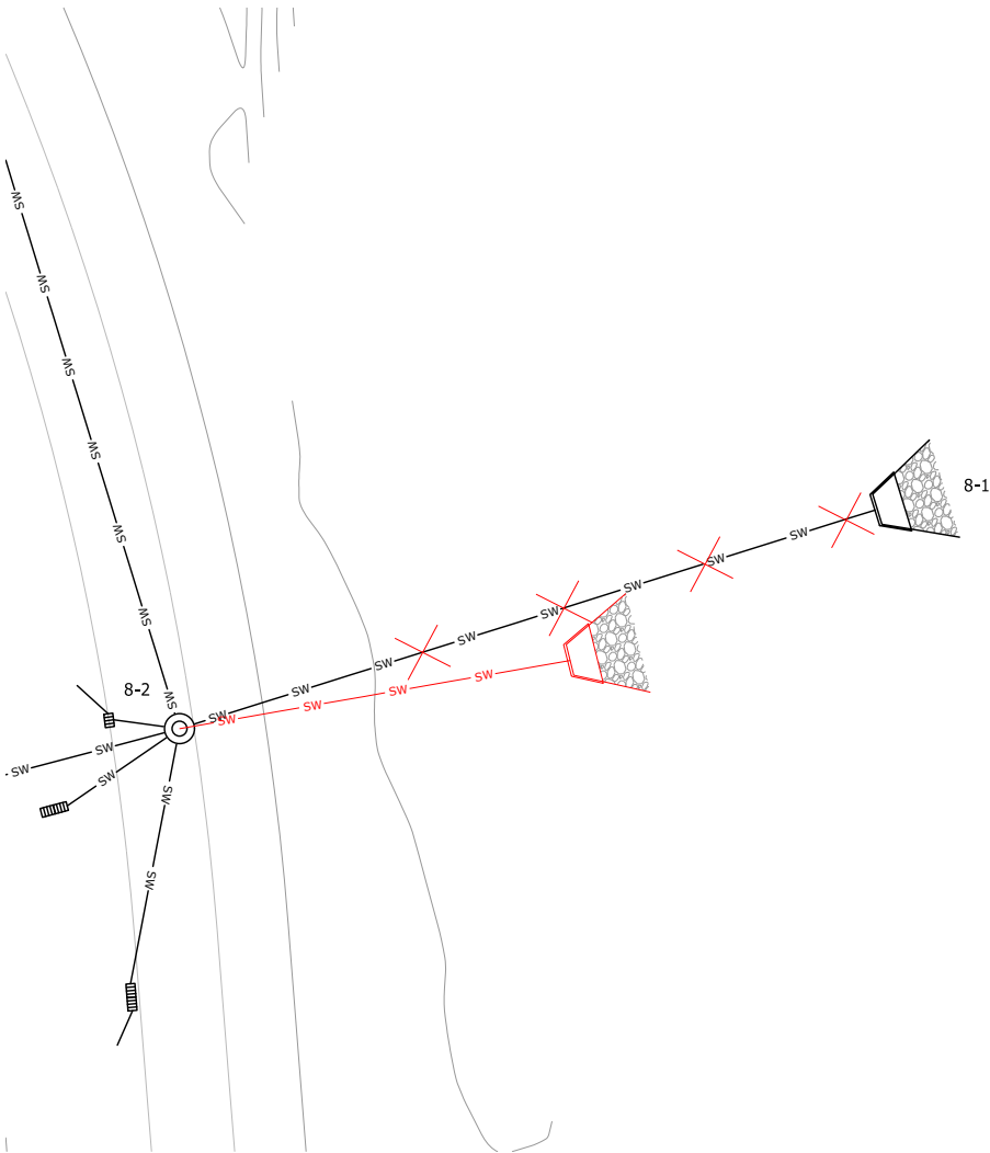
2 HEADWALL LAYOUT PLAN SK291 SCALE 1:250-A1 1:500-A3
