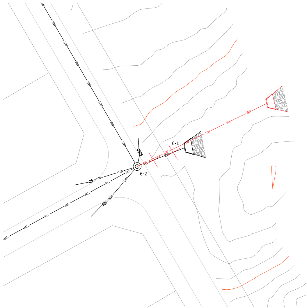
12 HEADWALL LAYOUT PLAN SK294 SCALE 1:250-A1 1:500-A3
