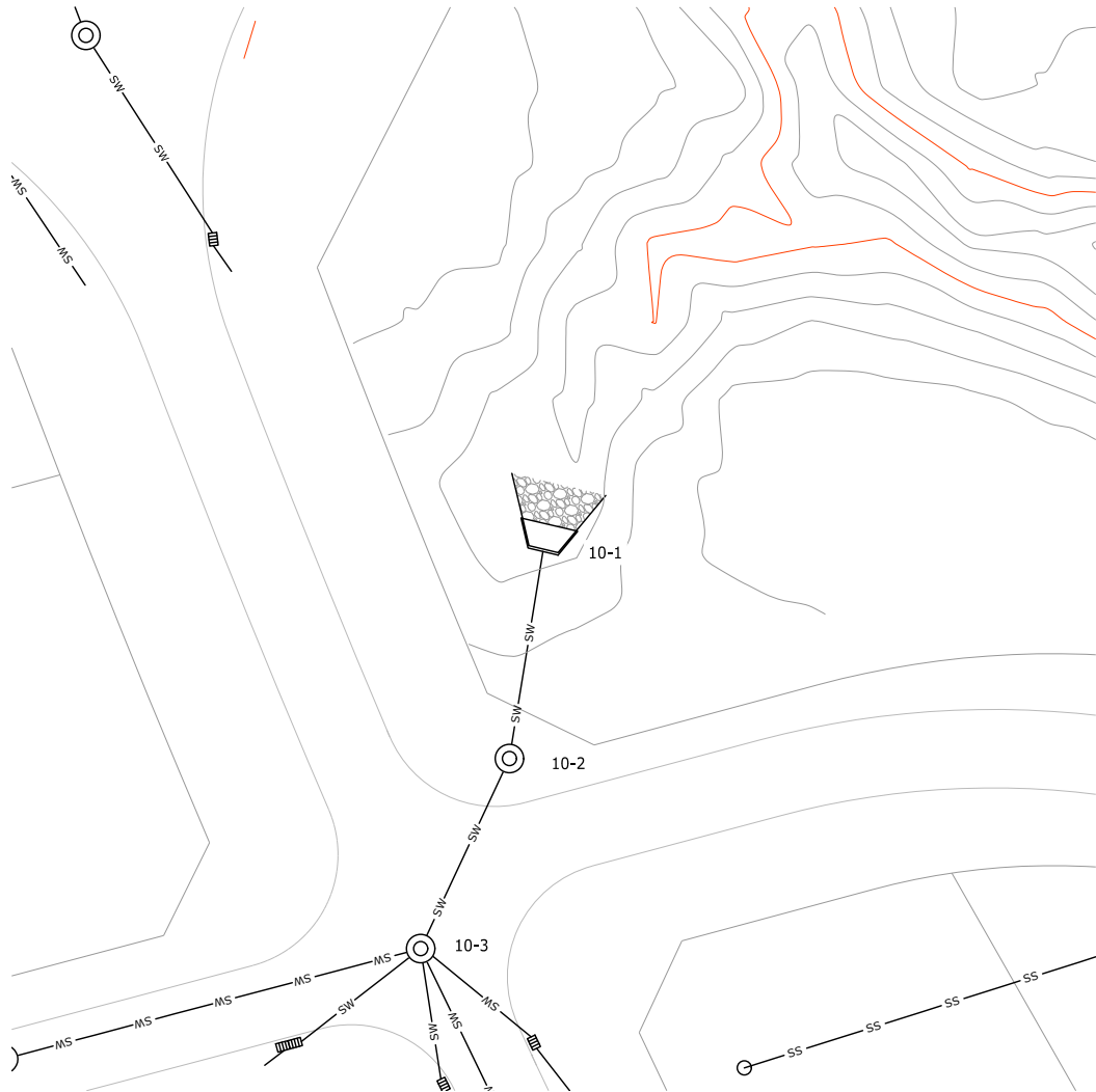
6 HEADWALL LAYOUT PLAN SK292 SCALE 1:250-A1 1:500-A3
