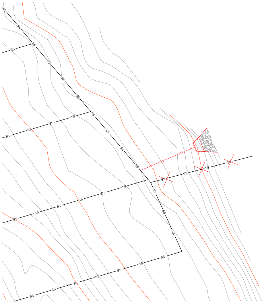
7 HEADWALL LAYOUT PLAN SK292 SCALE 1:250-A1 1:500-A3
