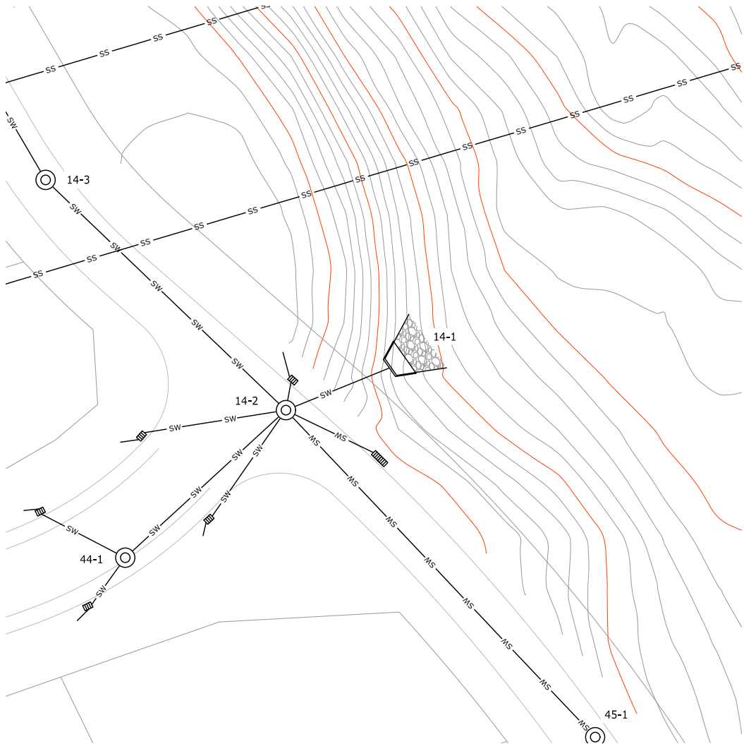
8 HEADWALL LAYOUT PLAN SK292 SCALE 1:250-A1 1:500-A3
