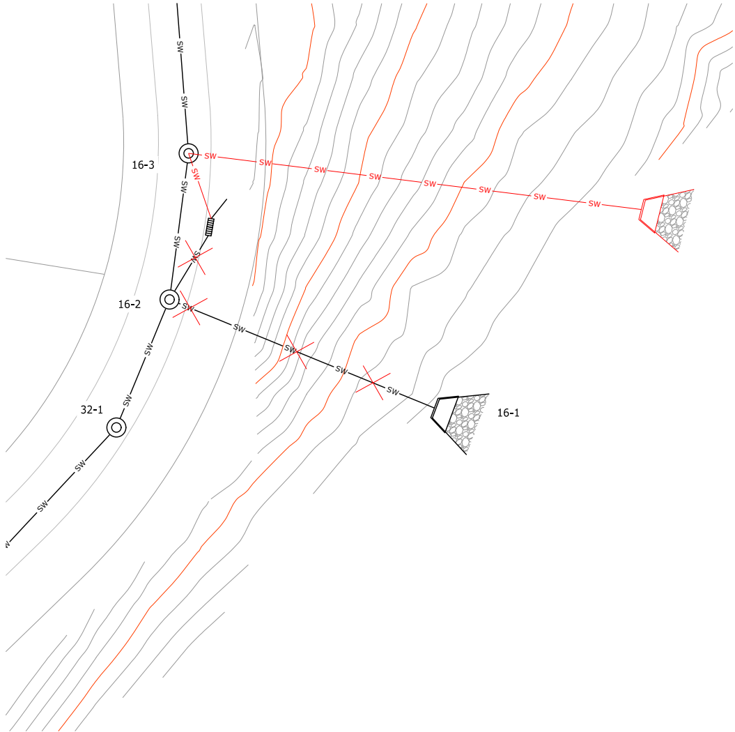
17 HEADWALL LAYOUT PLAN SK296 SCALE 1:250-A1 1:500-A3
