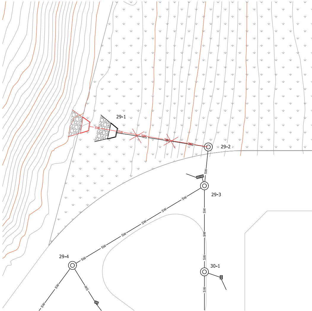
11 HEADWALL LAYOUT PLAN SK294 SCALE 1:250-A1 1:500-A3
